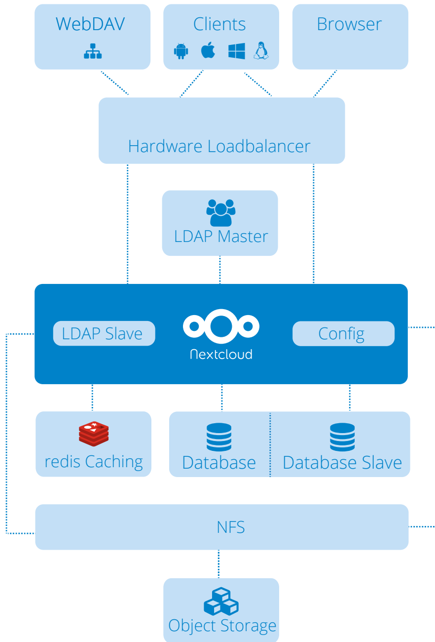
Figure 2: A scalable Nextcloud setup with NFS as storage layer, an LDAP user directory, REDIS caching servers, multiple database servers and a load balancer.
