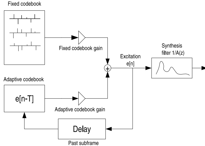
Figure 7.1.: The CELP model of speech synthesis (decoder)
